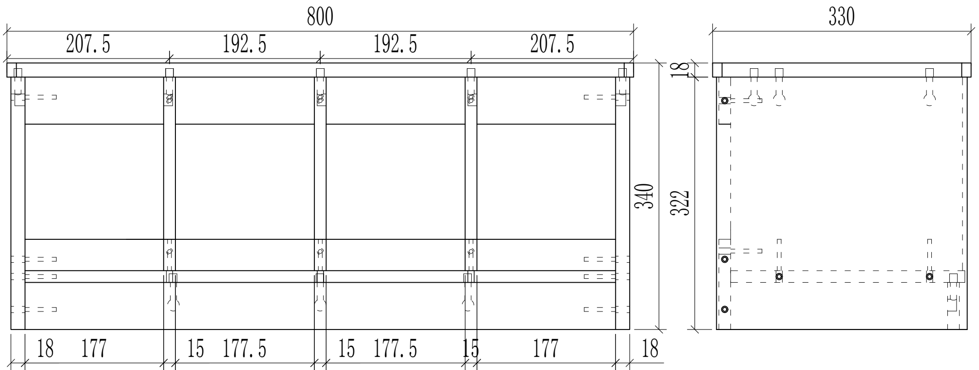
KB1-DG24119-30-F Cloakroom Bench 80-4-34
