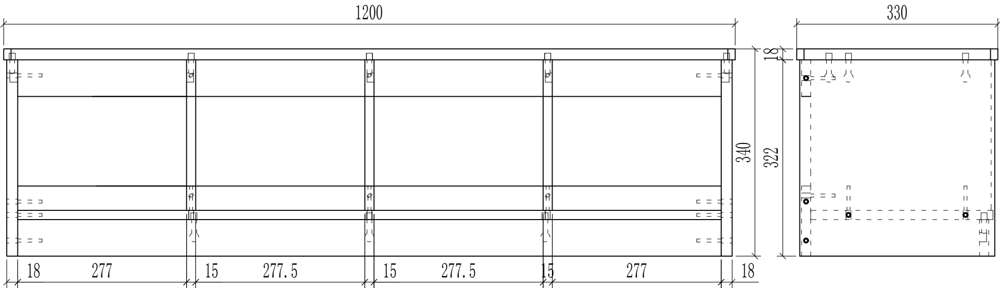
KB1-DG24125-30-F Cloakroom Bench 120-4-34
