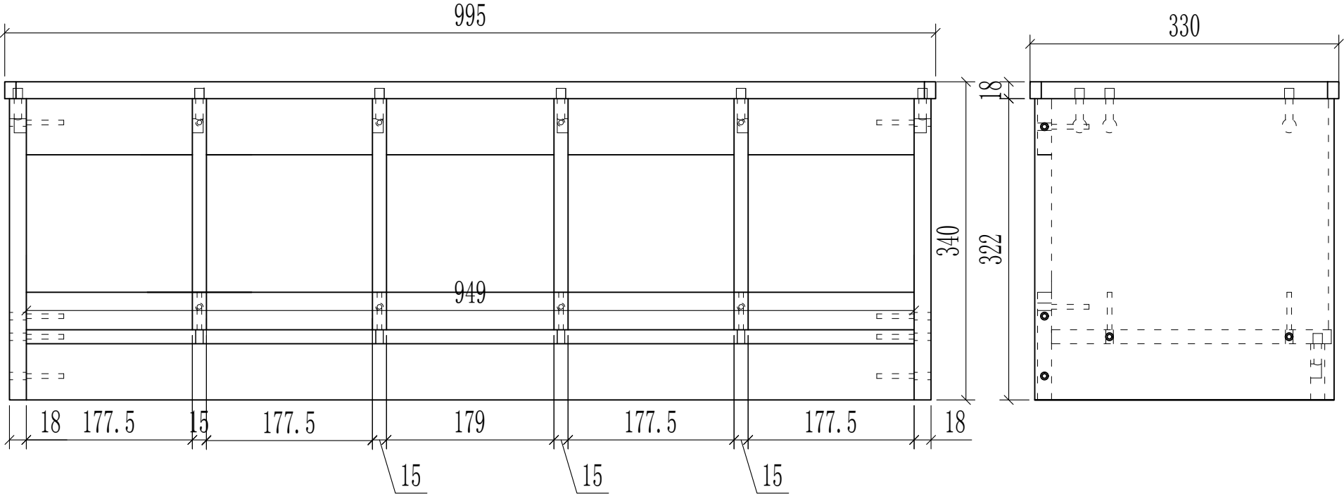
KB1-DG24123-30-F Cloakroom Bench 100-5-34
